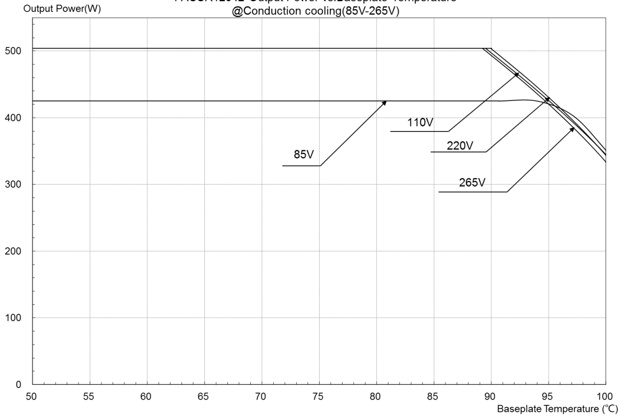
Figure 13: Thermal derating curves
