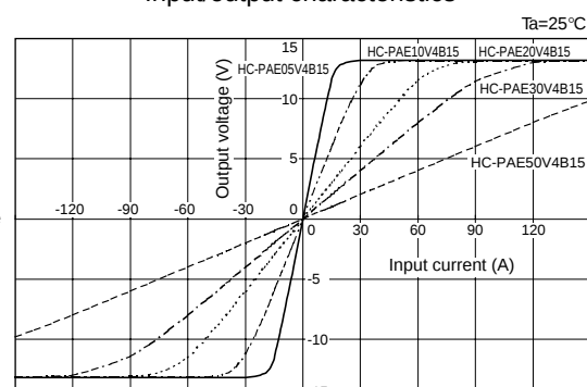
Input/output characteristics
