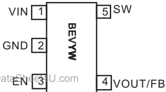
Top View SOT23-5
