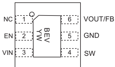
Top View DFN 2x2 6L
