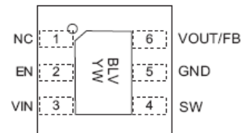
Top View DFN 2x2 6L
