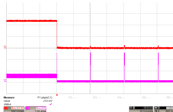
(CH3=Output Voltage; CH4=Inductor Current)
