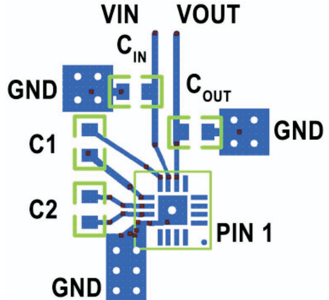
Figure 4: PCB layout
