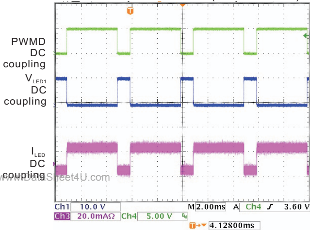
LED Current Waveforms (PWMD=80%)
