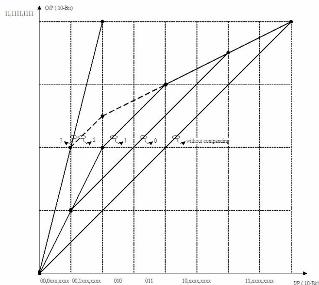
Figure 3.2 Companding curves program by Compaund_EnH and Compaund_Sel
