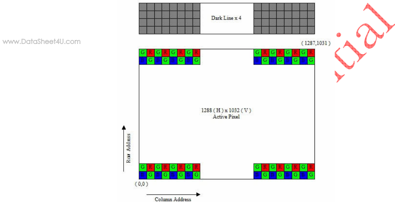
Figure 2.1 Physical Sensor Array Format
