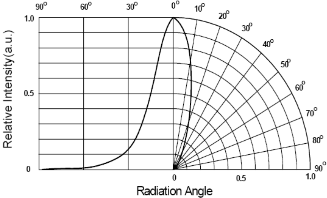
Figure 14. Radiation Characteristics
