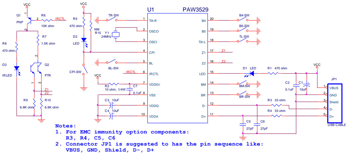
Figure 13. 4D5B Application Circuit with IRPTR Zwheel.
