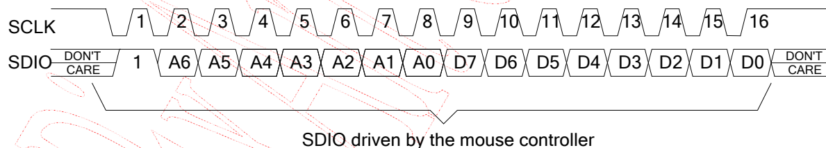
Figure10. Write Operation
