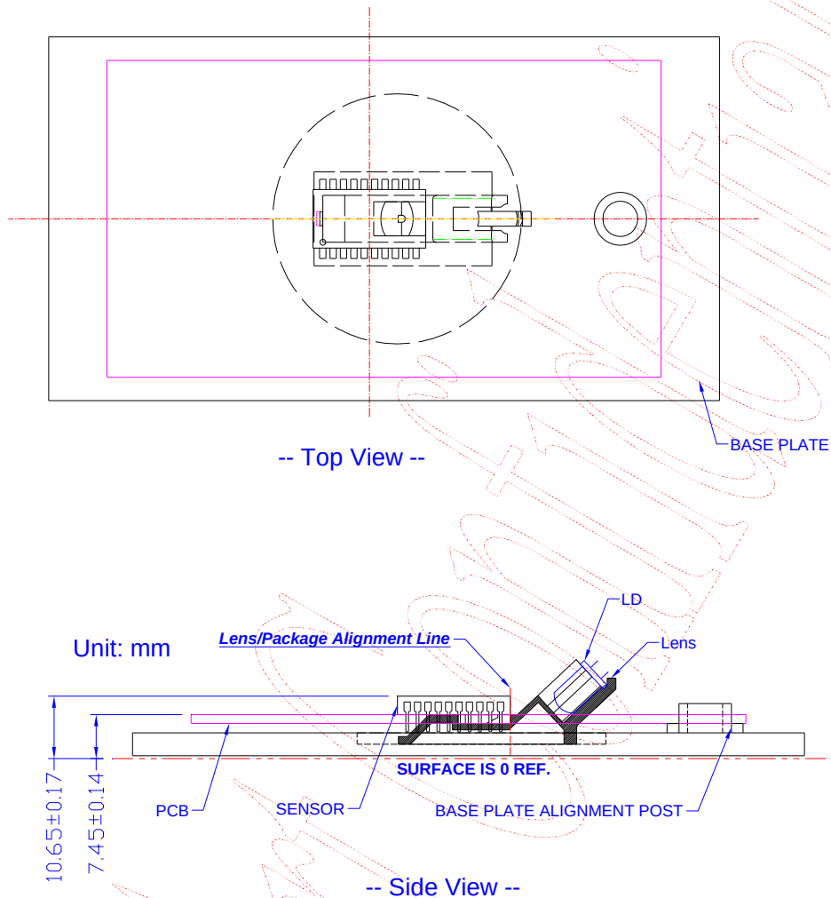
Figure 4. 2D Assembly
