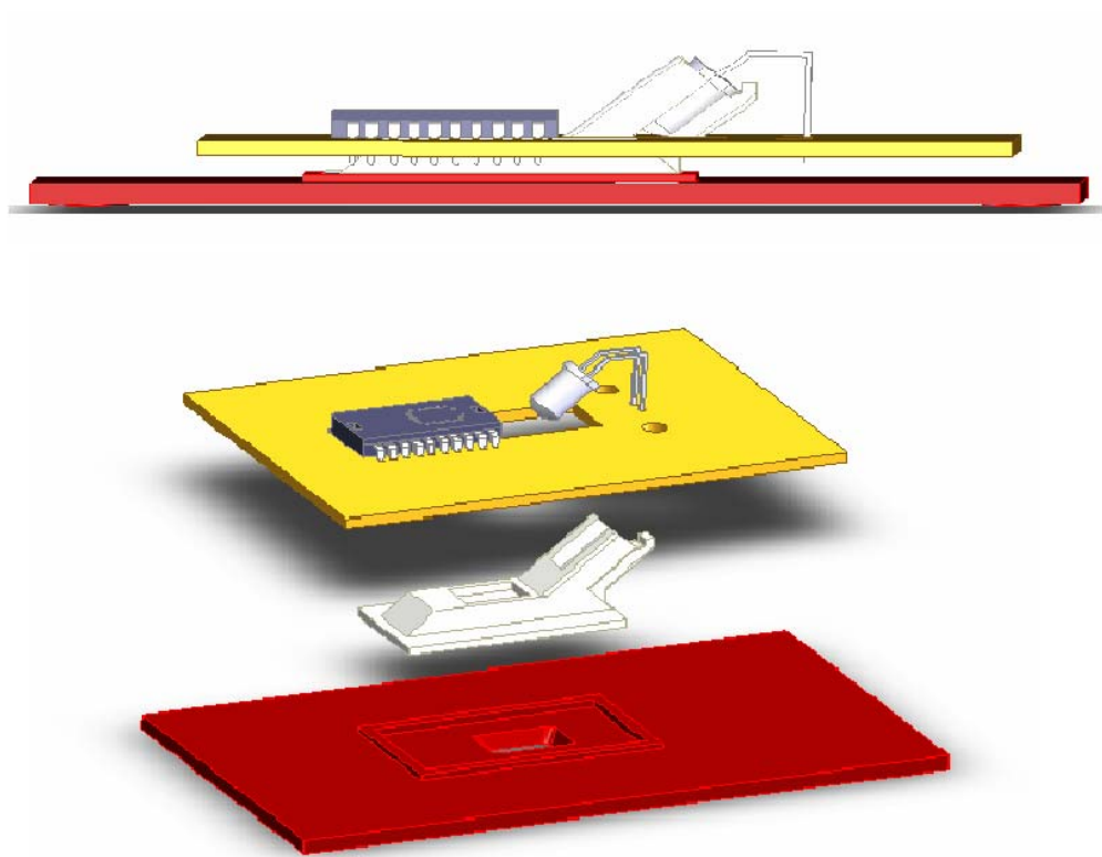
Figure 5. 3D Assembly
