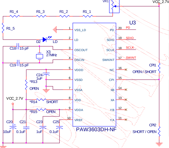
Figure 17. Application Circuit for 2.7V
