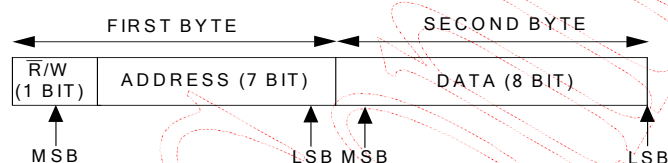
Figure 9. Transmission Protocol
