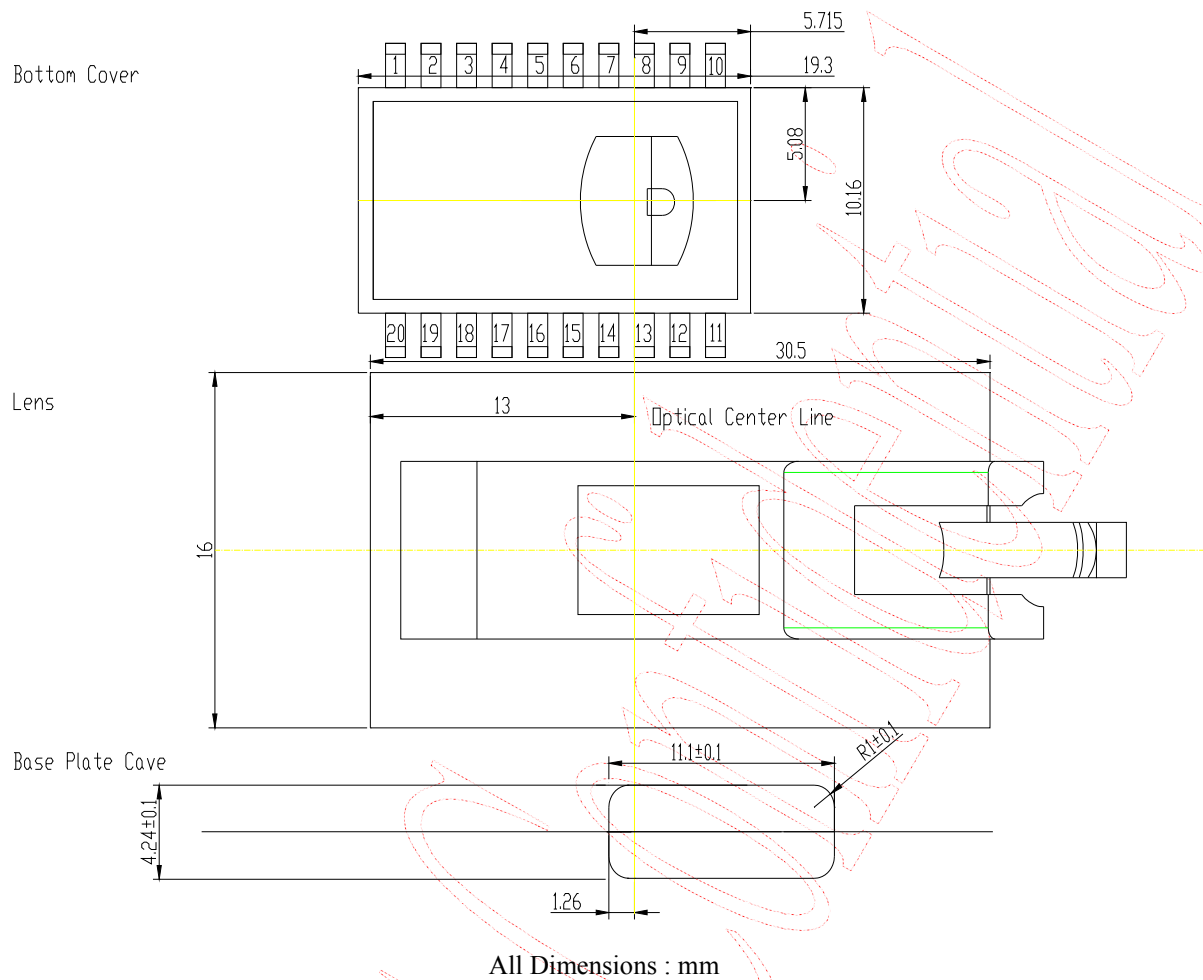
Figure 21. Base Plate Molding Dimension
