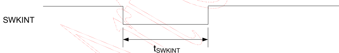
Figure 16. SWKINT Timing
