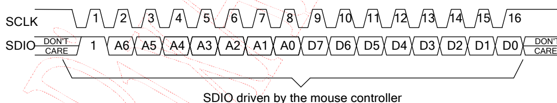
Figure 10. Write Operation
