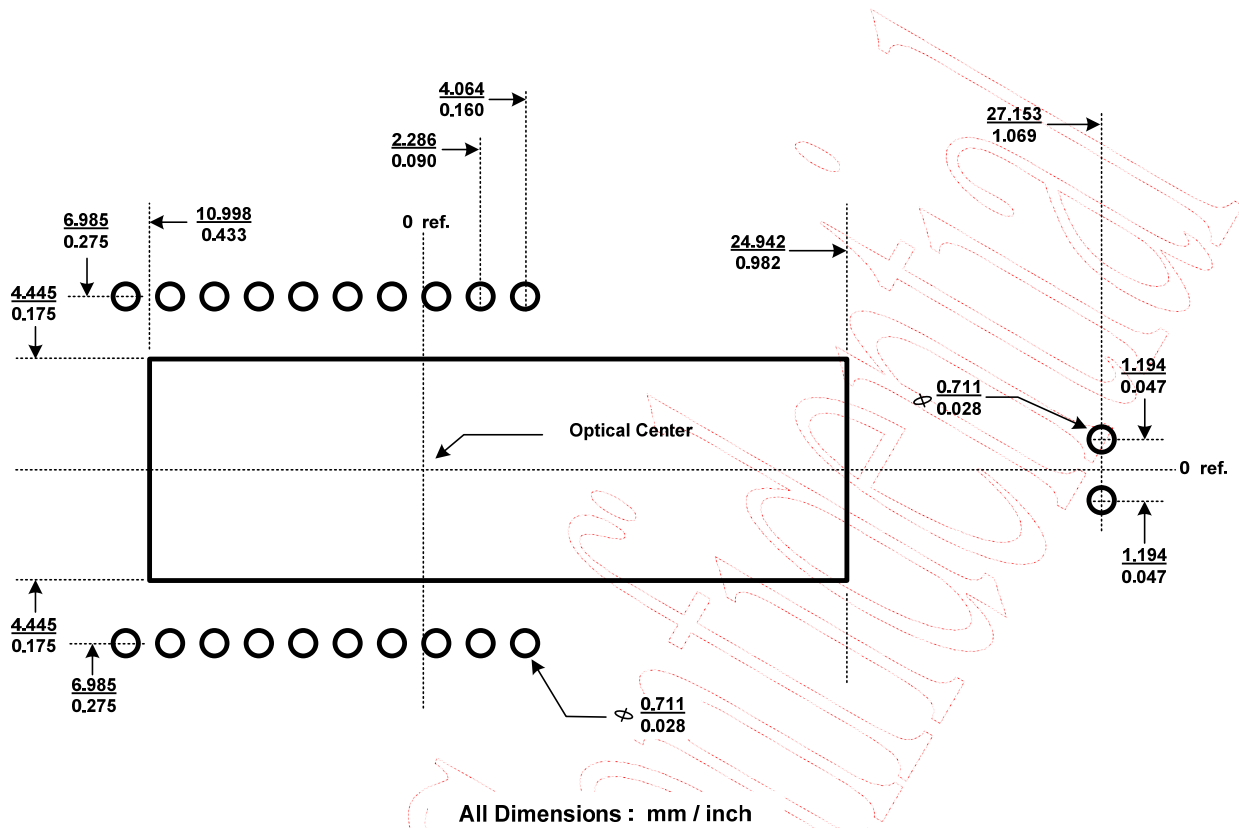
Figure 22. Recommended PCB Mechanical Cutouts and Spacing
