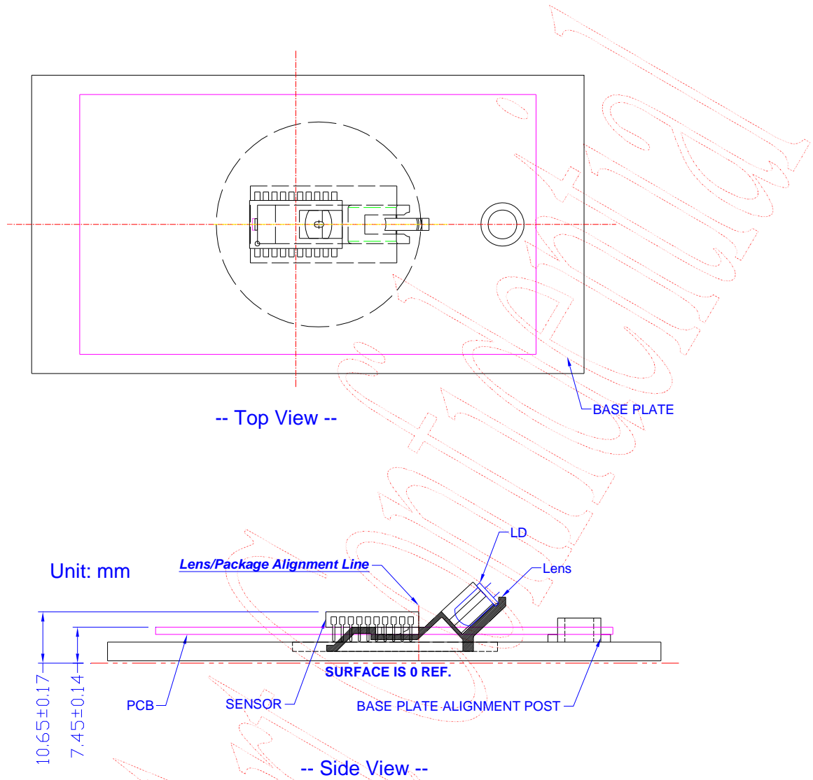
Figure 4. 2D Assembly
