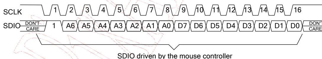
Figure 10. Write Operation
