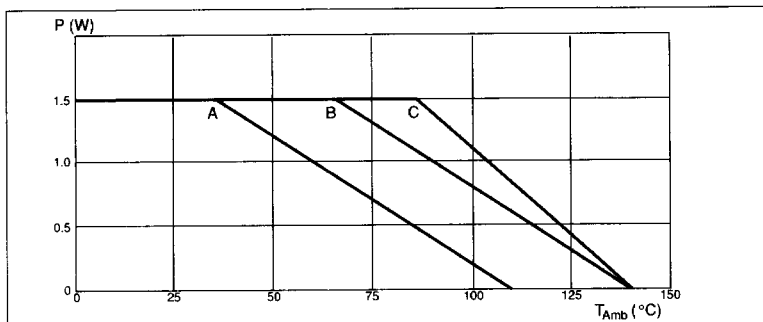
Figure 13. Power derating.
