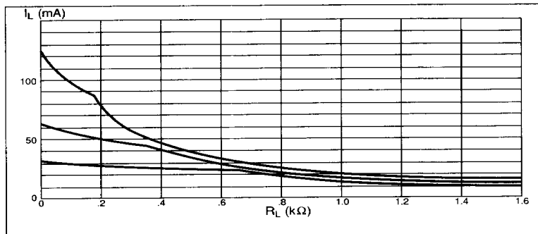
Figure 14. Examples of PBL 3762 loop feed. R_{SG} \rightarrow \infty , V_{Bat} = -28\text{V} .
