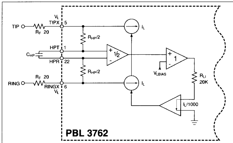
Figure 9. Longitudinal impedance.
