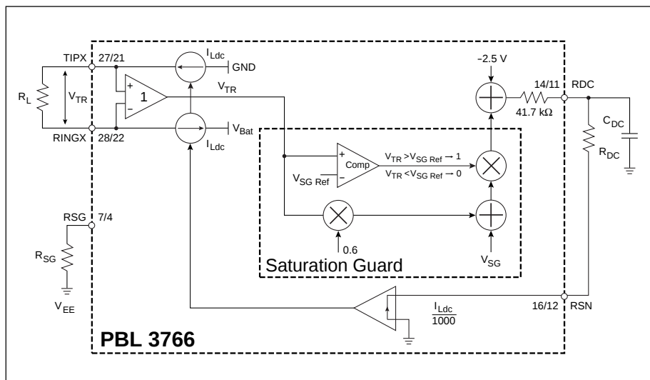
Figure 12. Battery feed ( C_2, C_1 = 1, 0 ; active state).
