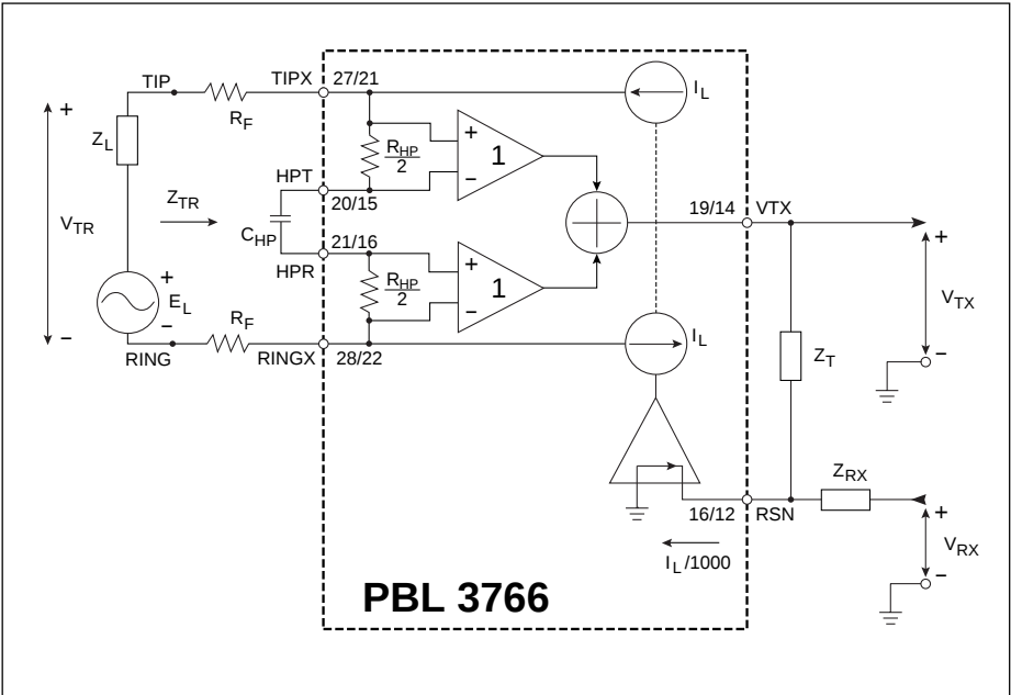
Figure 8. Simplified ac transmission circuit.
