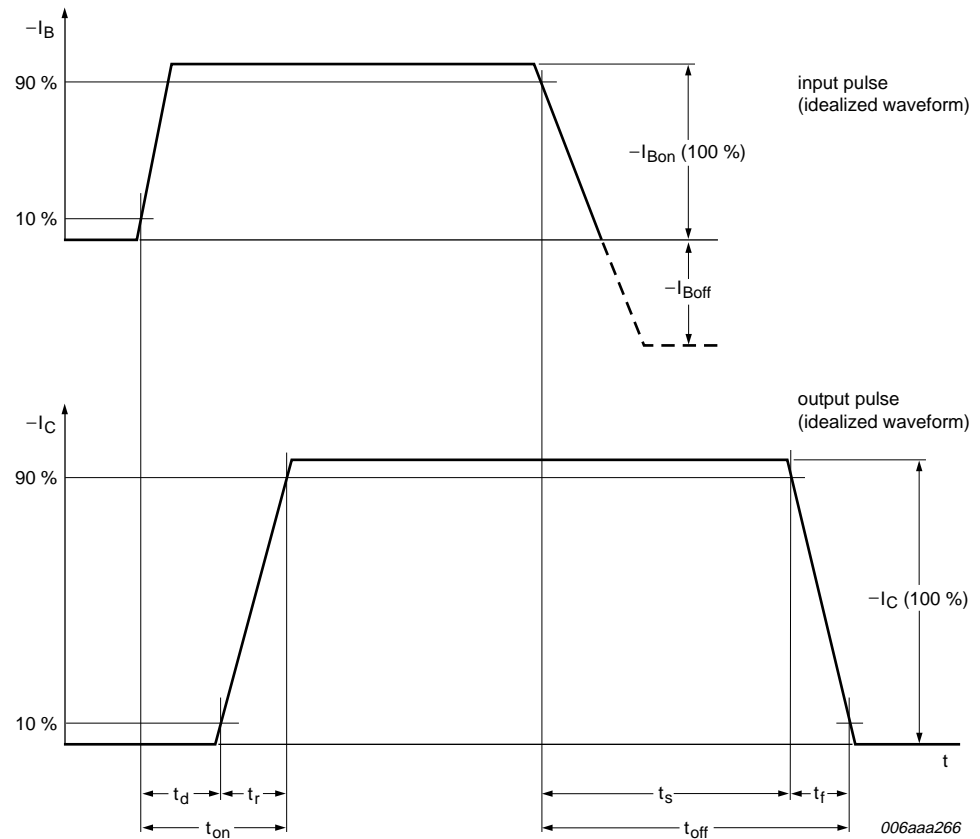
Fig 17. BISS transistor switching time definition
