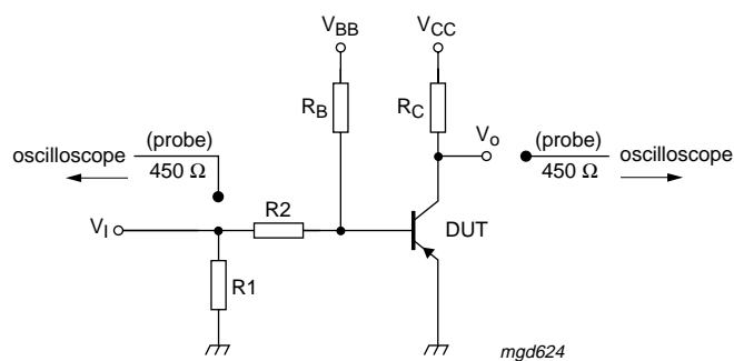
Fig 18. TR1: BISS transistor switching time definition
