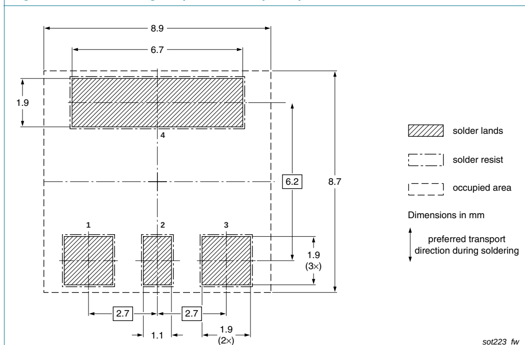
Fig 17. Wave soldering footprint SOT223 (SC-73)
