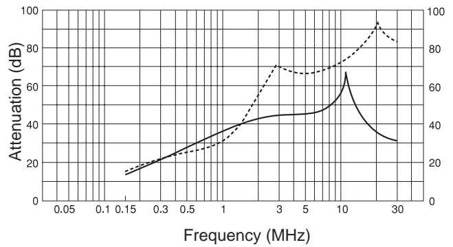
PBW-1206-33
