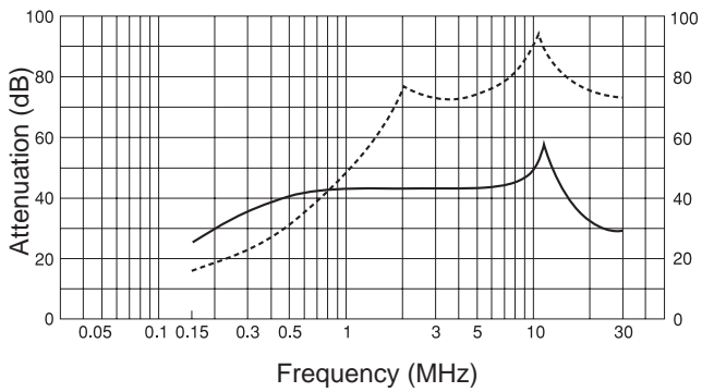
PBW-1203-33
