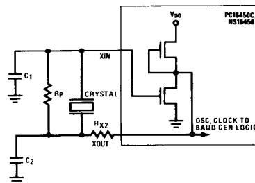
Typical Oscillator Networks
