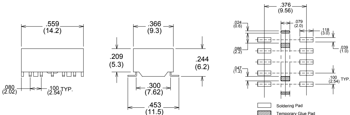
Single Side Stable
