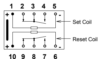
Dual Coil Latching
