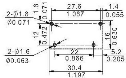
Mounting (Bottom view)
