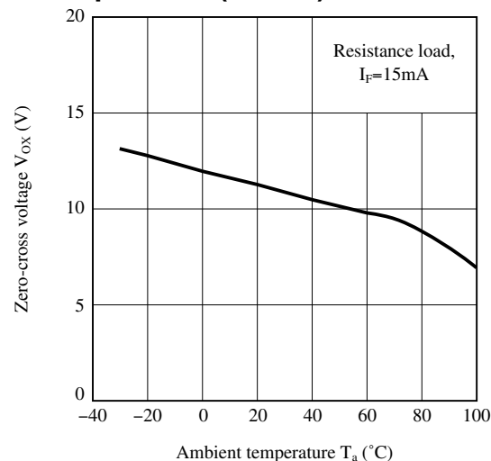
Fig.9 Zero-cross Voltage vs. Ambient Temperature (rank B)
