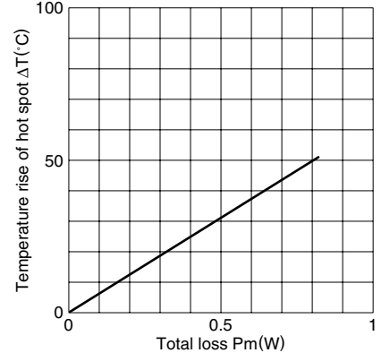
Temperature rise vs. Total loss for EPC13 core (Typical) (Ambient temperature: 25°C)
