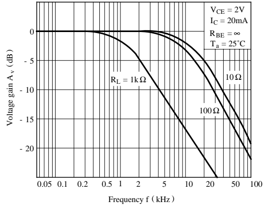
Fig.10 Frequency Response
