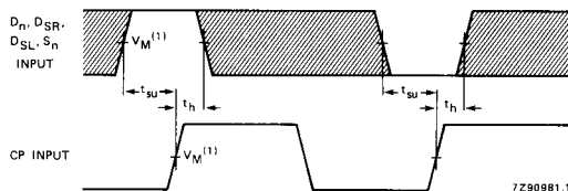
Fig. 8 Waveforms showing the set-up and hold times from the D_n , D_{SR} , D_{SL} and S_n inputs to the clock (CP).
