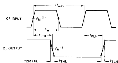
Fig. 6 Waveforms showing the clock (CP) to output ( Q_n ) propagation delays, the clock pulse width, the output transition times and the maximum clock frequency.
