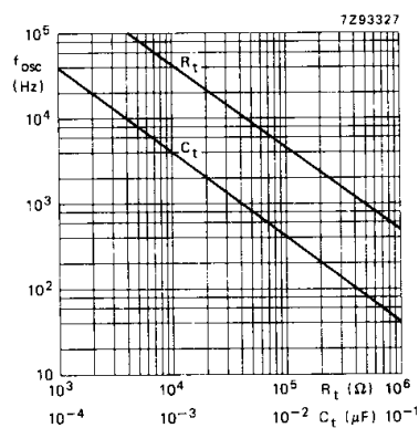
Fig. 9 RC oscillator frequency as a function of R_t and C_t at V_{CC} = 2.0 to 6.0 V; T_{amb} = 25^\circ C .
