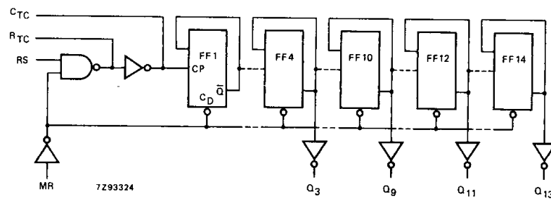
Fig. 5 Logic diagram.
