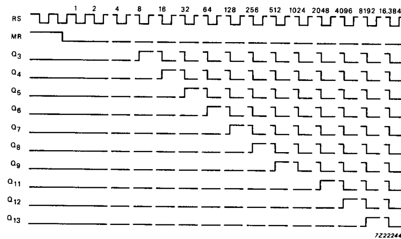
Fig. 6 Timing diagram.
