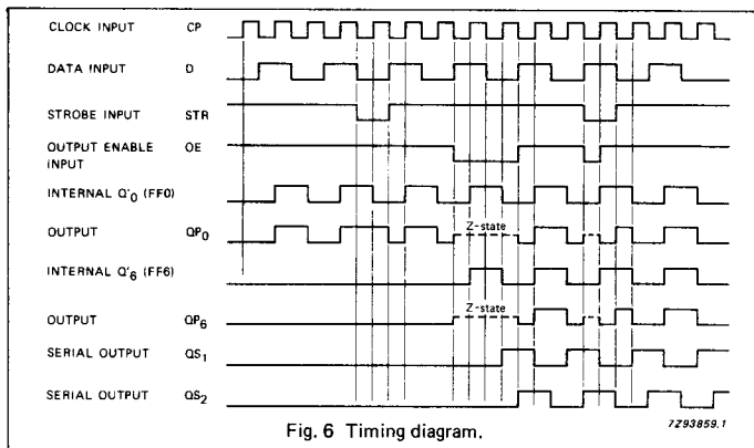
Fig. 6 Timing diagram.
