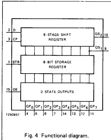
Fig. 4 Functional diagram.
