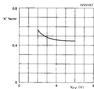
Fig. 10 Typical 'K' factor; external capacitance = 10 \text{ nF} , external resistance = 10 \text{ k}\Omega to 100 \text{ k}\Omega and T_{amb} = 25^\circ\text{C} .
