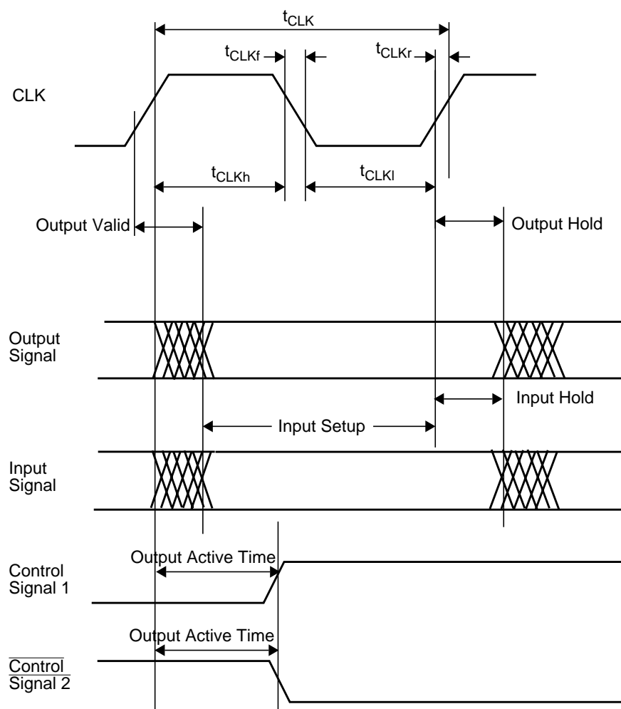
Figure 132. Clock Waveforms
