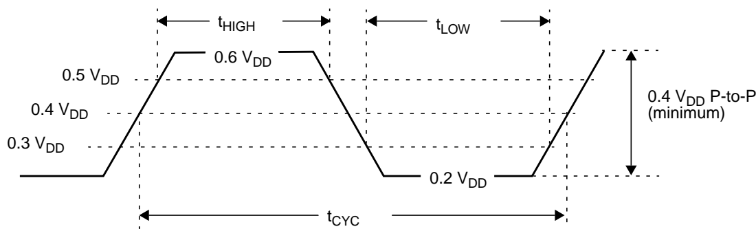
Figure 166. LCLK Waveform
