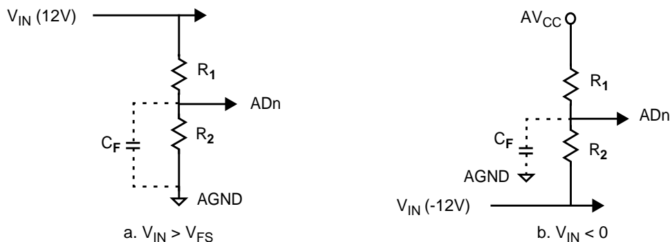
Figure 61. Measurement of Positive and Negative Voltages
