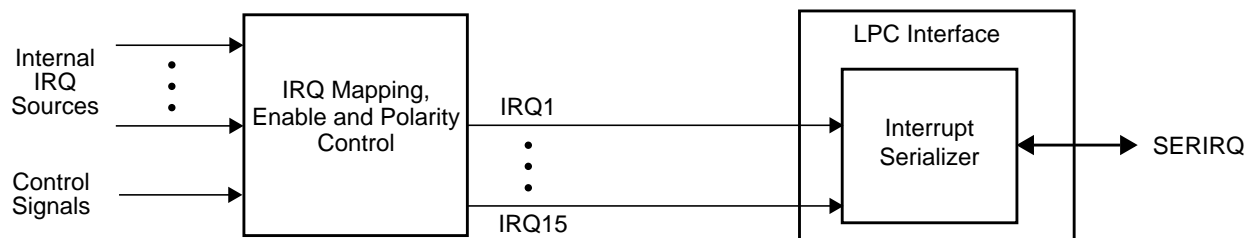
Figure 111. Interrupt Serialization Mechanism
