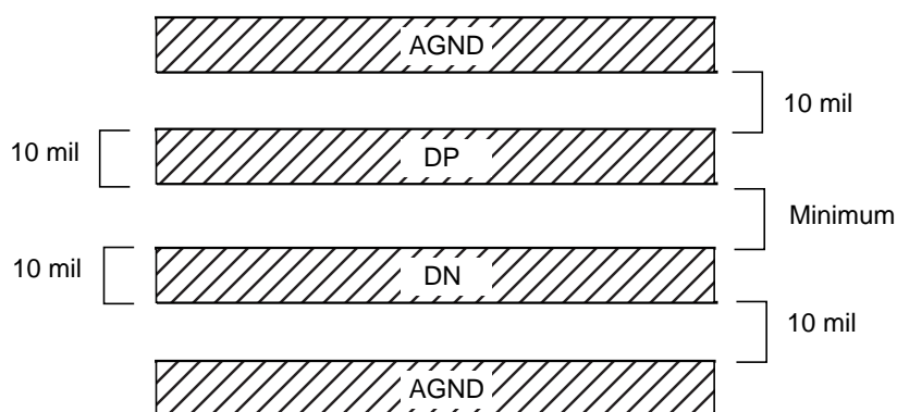
Figure 65. DP and DN, PCB Traces
