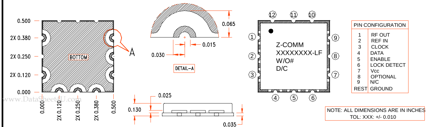
PHYSICAL DIMENSIONS
