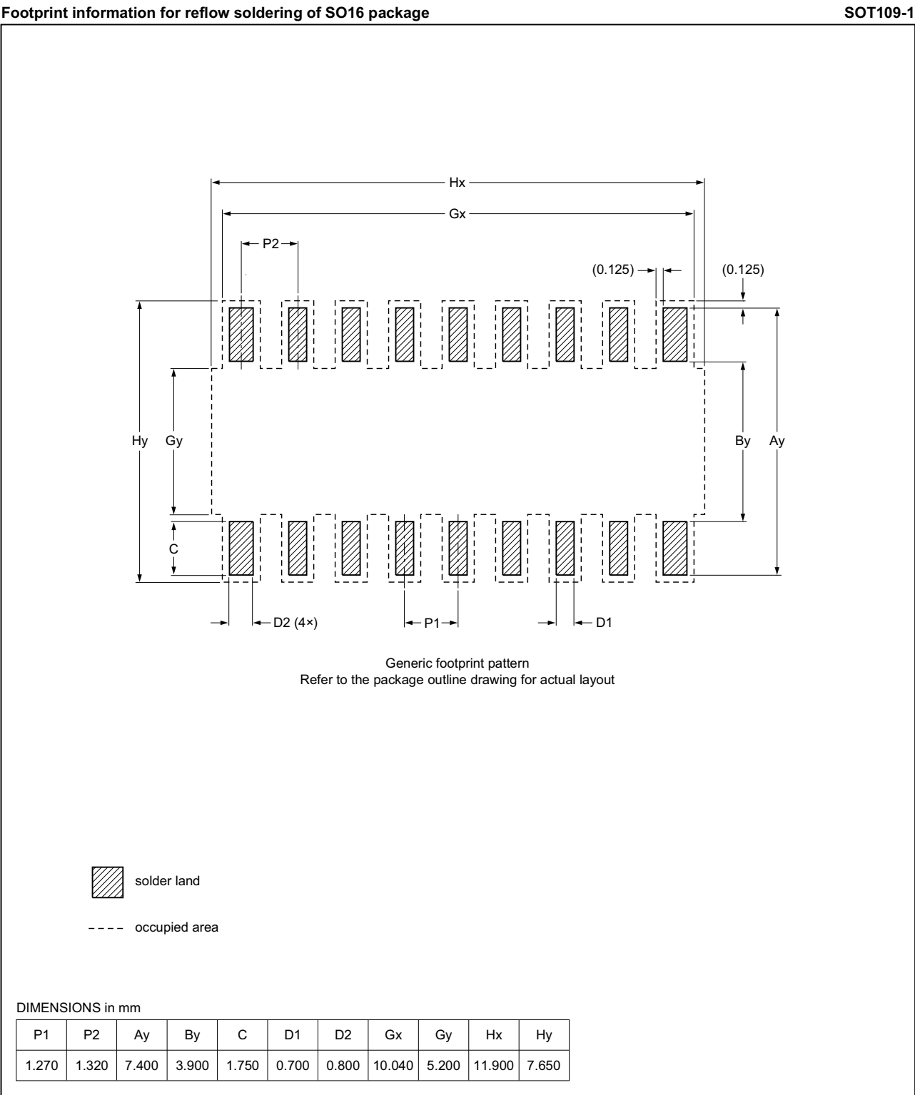
Fig 31. PCB footprint for SOT109-1 (SO16); reflow soldering
