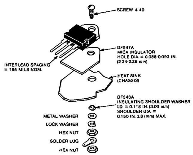
Suggested mounting hardware for JEDEC TO-218AC
