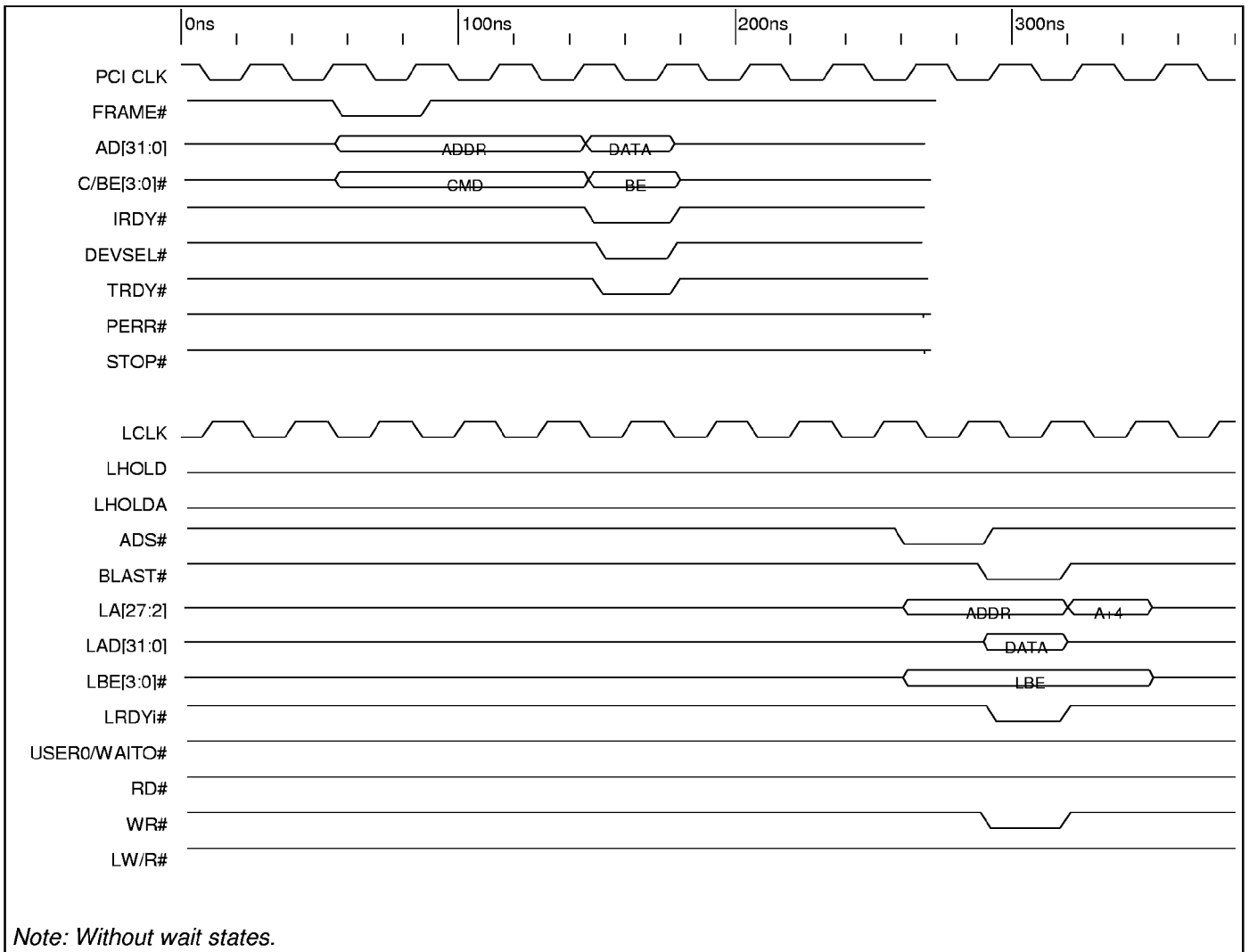
Timing Diagram 8-8. Direct Slave Single Write (32 Bit Local Bus)
