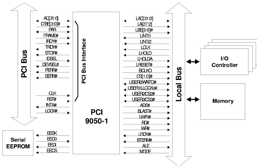
Figure 1-1. PCI 9050-1 Block Diagram
