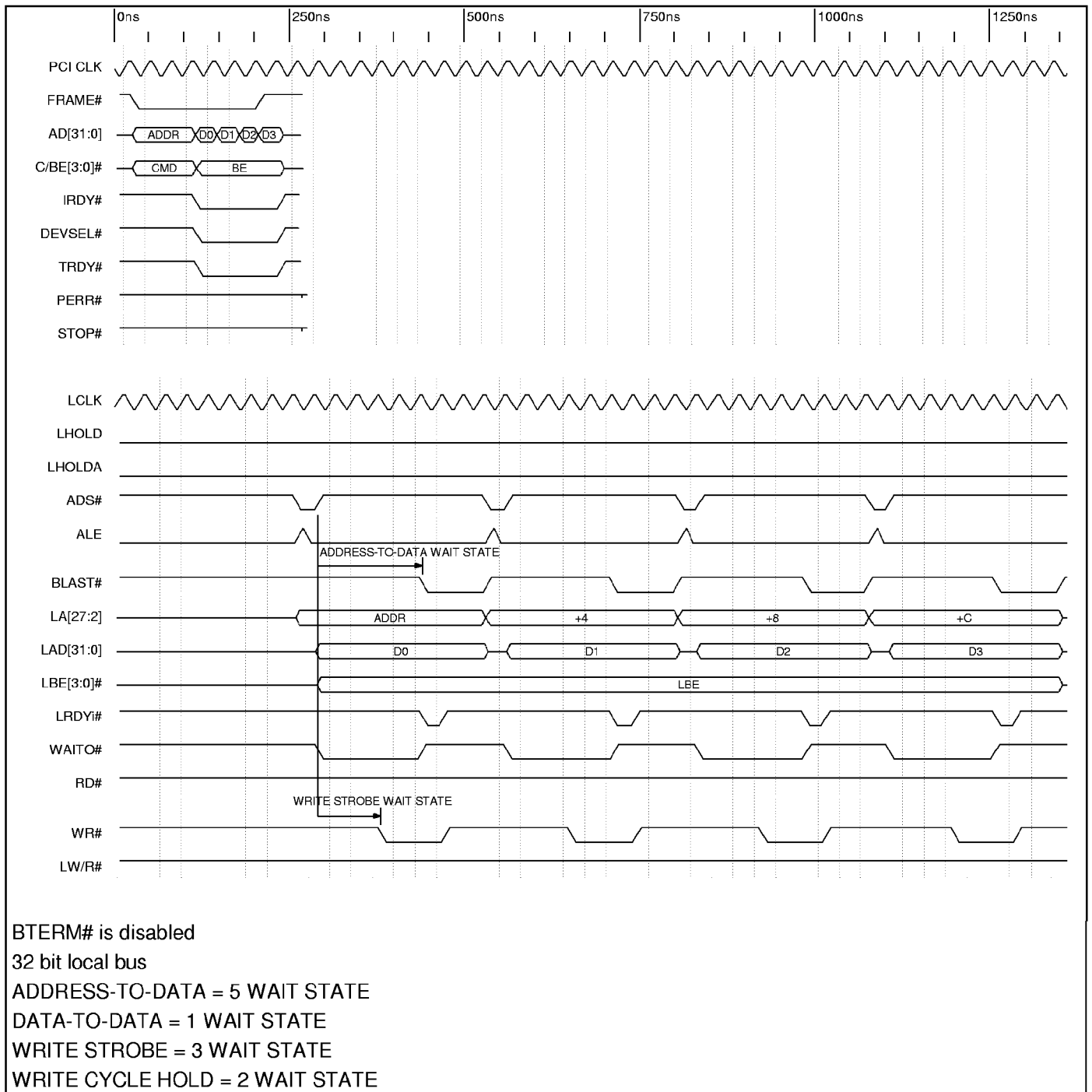
Timing Diagram 8-9. Direct Slave Non-Burst Write with Wait States (32 Bit Local Bus)
