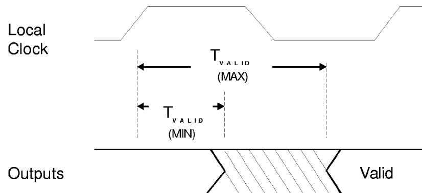
Figure 6-1. PCI 9050 Local Output Delay
