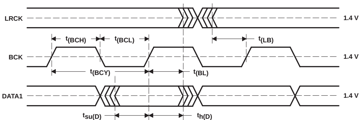
Figure 4. Bit Clock Timing for TDM Format
