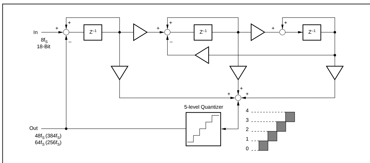
FIGURE 11. 5-Level \Delta\Sigma Modulator Block Diagram.
