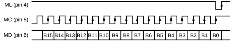
FIGURE 5. Serial Interface Timing.
