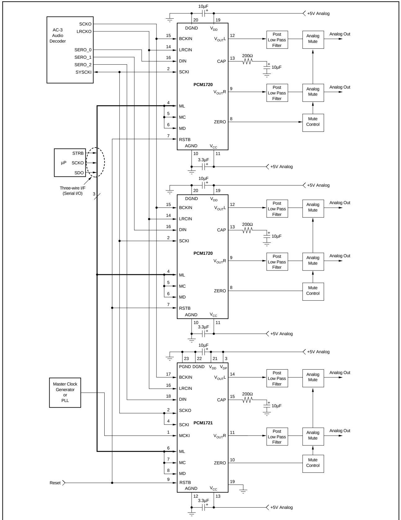
FIGURE 13. Connection Diagram for a 6-Channel AC-3 Application.
