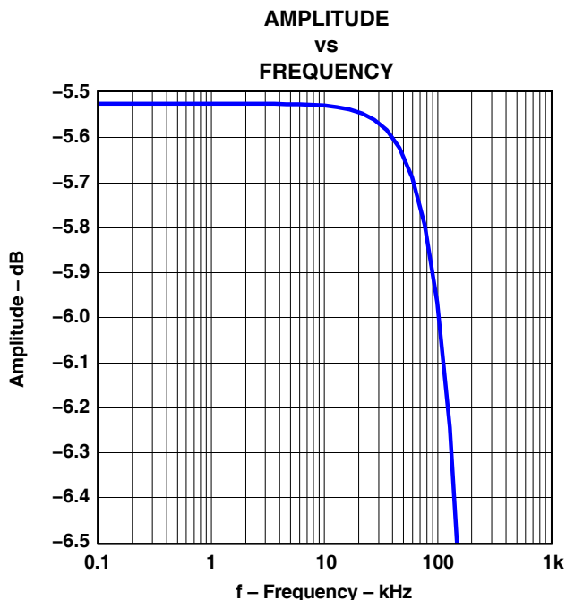
Figure 7. Antialiasing Filter Pass-Band Characteristics
