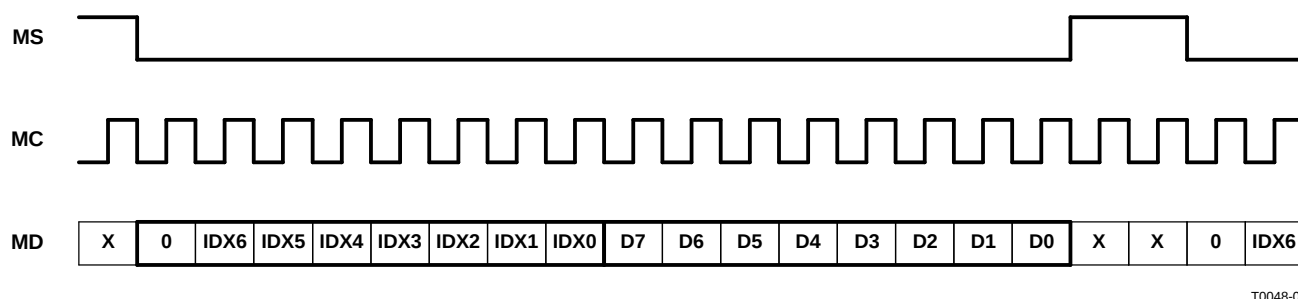
Figure 28. Serial Control Format
