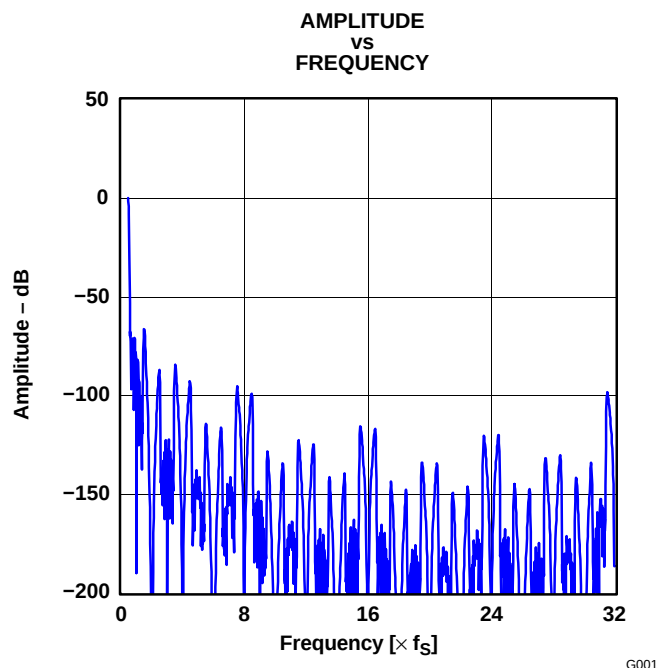
Figure 1. Overall Characteristics
