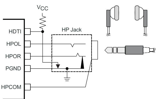
Figure 42. Connection for Headphone Output and Insertion Detection
