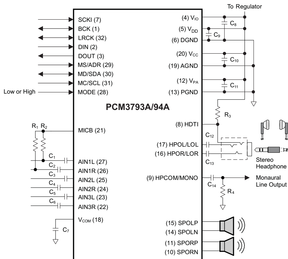
Figure 40. Connection Diagram
