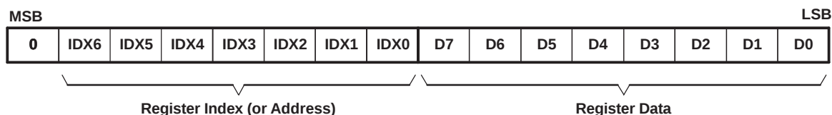
Figure 30. Control Data Word Format for MD
