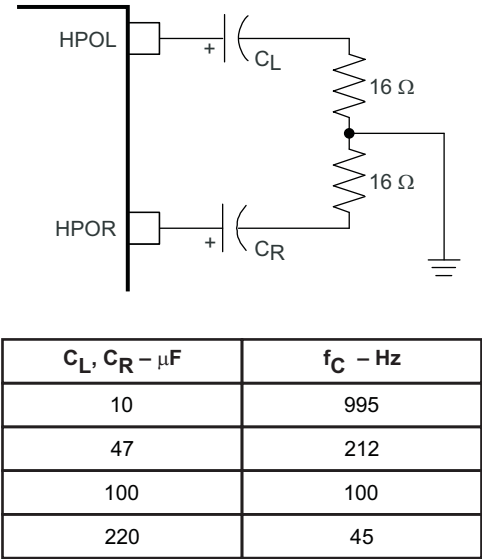
Figure 43. High-Pass Filter for Headphone Output
