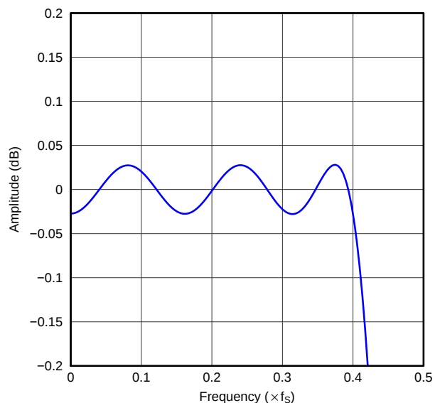
Figure 41. Asymmetric FIR x8 Interpolation Filter Passband Ripple, Single Rate
