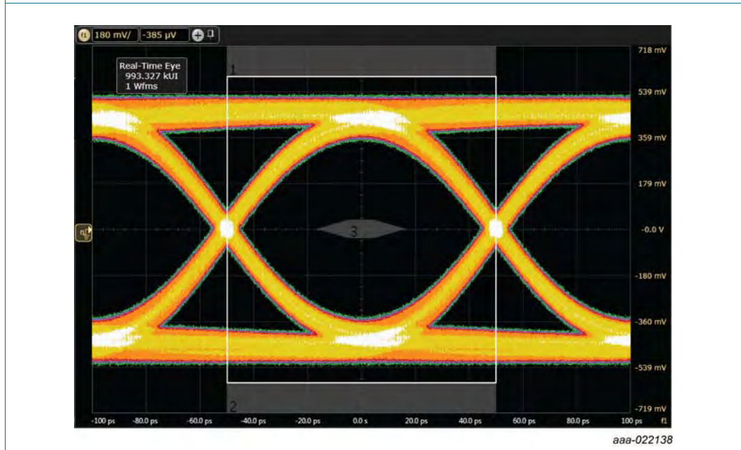
Fig 5. USB 3.1 eye diagram, test board with PCMF2USB30; typical values
