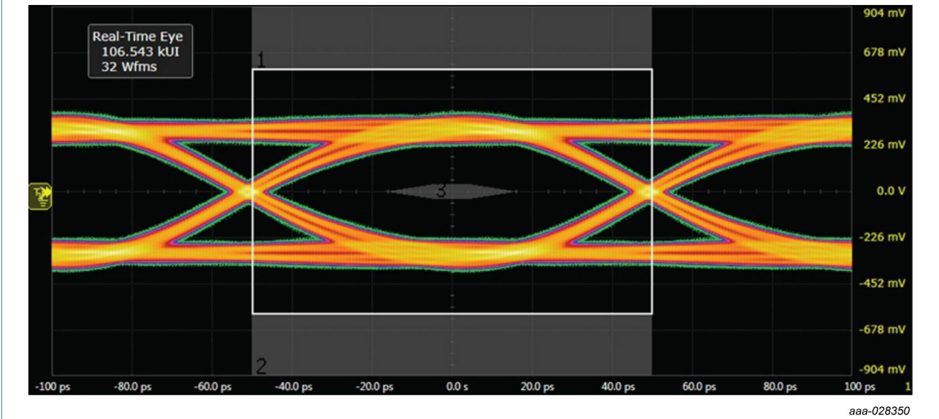
Fig. 6. USB 3.2 eye diagram 10 Gbps, test board without device; typical values
