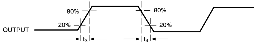
Figure 3. All Outputs Rise/Fall Time
