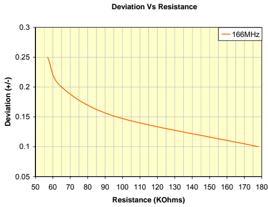
Fig19: Deviation Vs Resistance (166MHz, FS=1)
