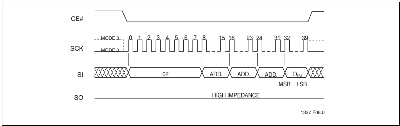
FIGURE 7: Byte-Program Sequence
