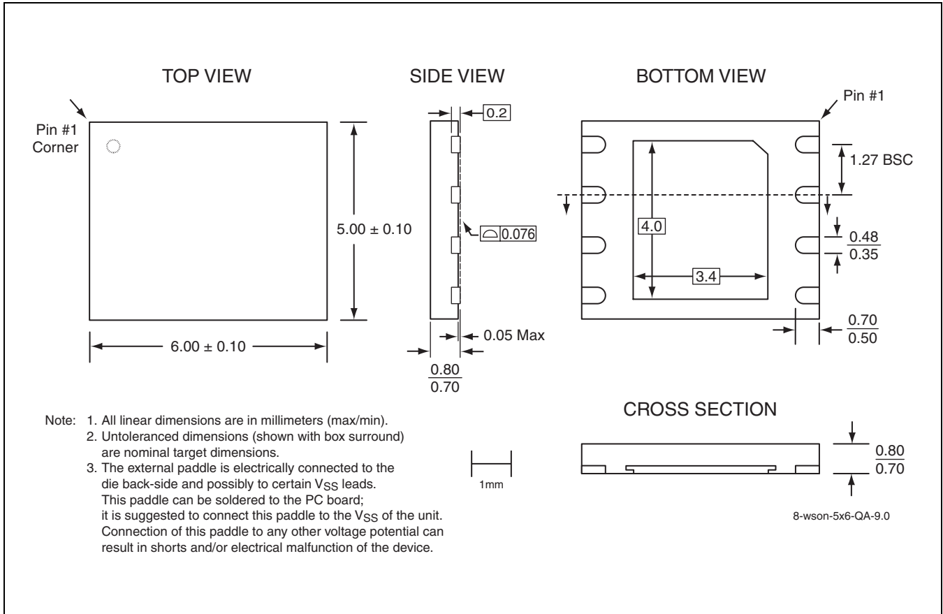
FIGURE 28: 8-Contact Very-very-thin, Small-outline, No-lead (WSON) PCT Package Code: QA
