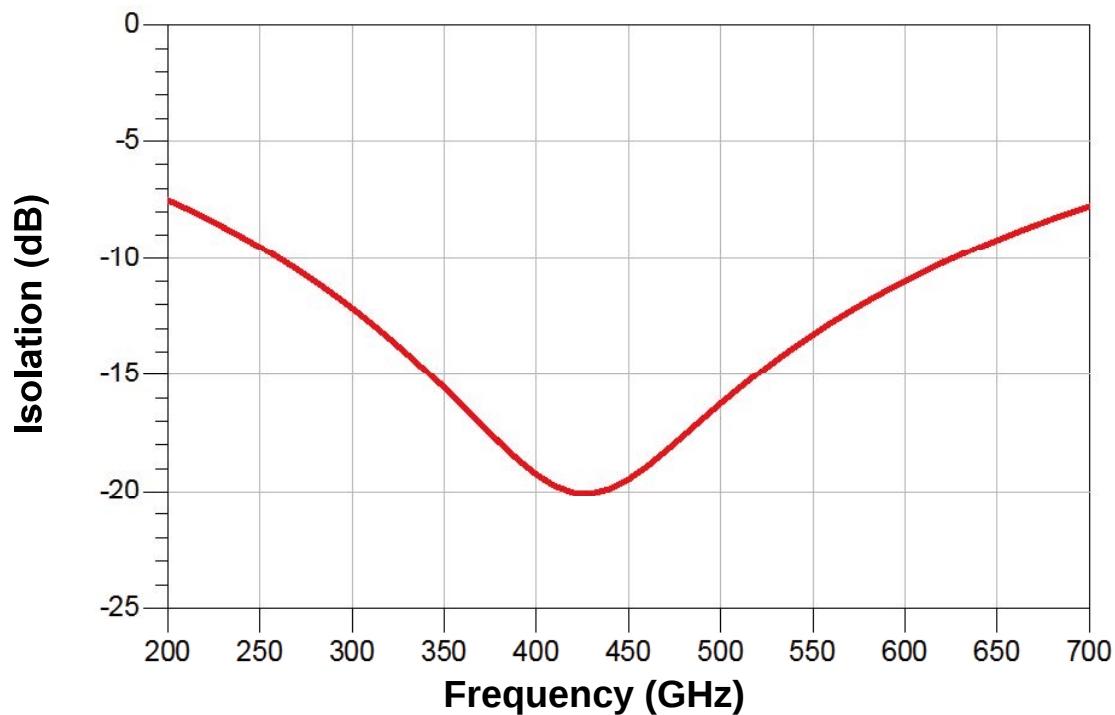
Isolation VS.Frequency
