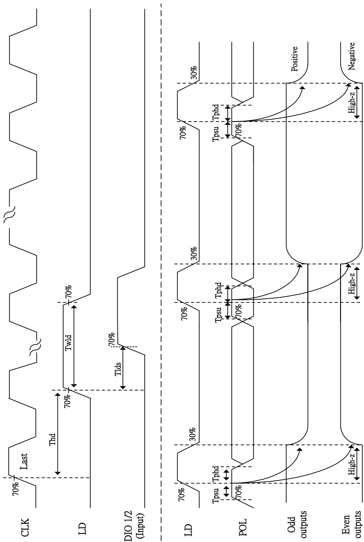
Fig. 11-2 Horizontal timing(2)
