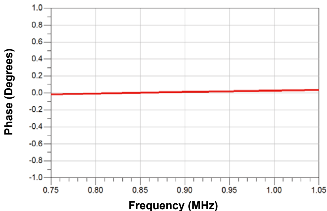
Phase Balance VS.Frequency
