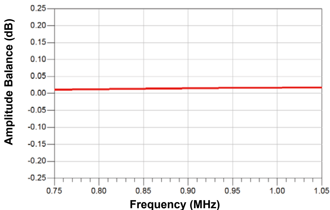
Amplitude Balance VS.Frequency
