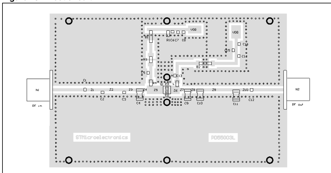
Figure 16. Test circuit
