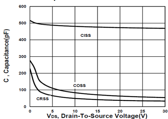
Capacitance Characteristic
