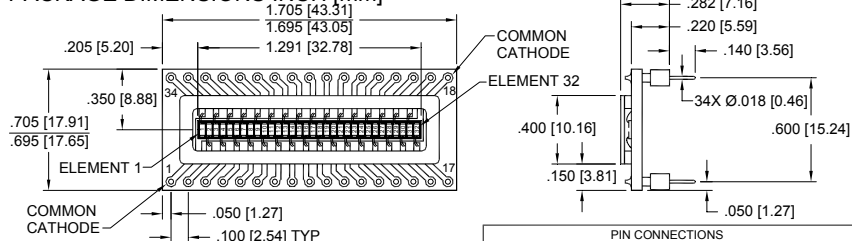
PIN CONNECTIONS
