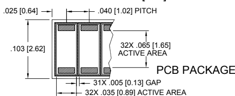
CHIP DIMENSIONS INCH [mm]
